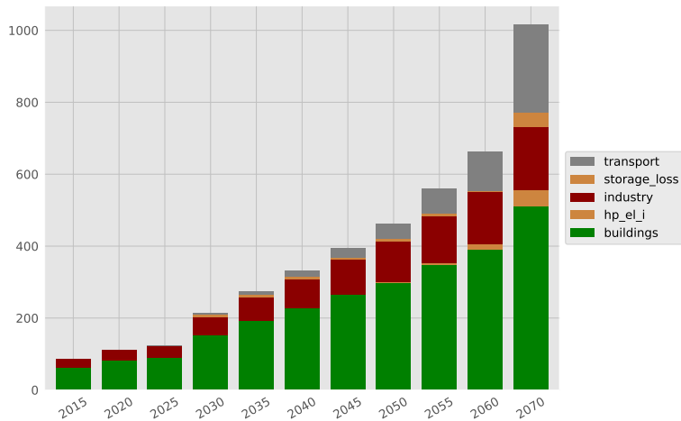
Electricity use (TWh)
