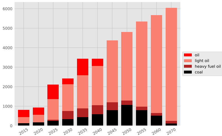
Energy imports (PJ)
