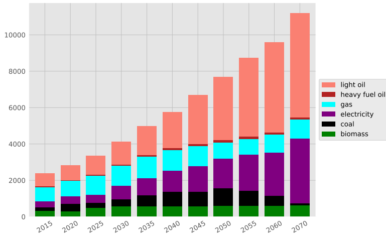
Final energy consumption (PJ)
