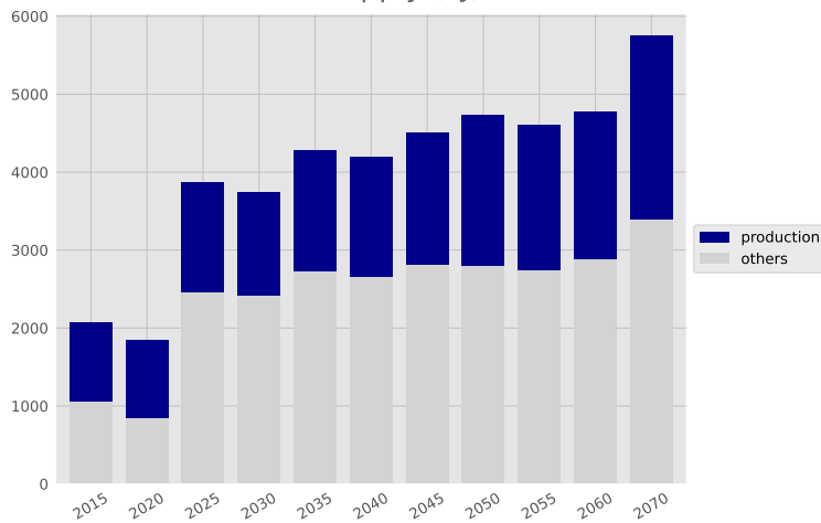
Gas supply (PJ)
